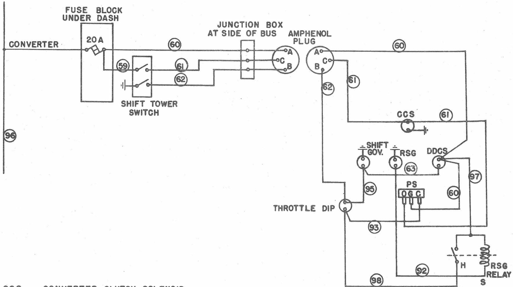
THROTTLE DIP CIRCUIT 8200-8349
